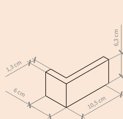
VICTORIAN HALF BRICK CORNER
