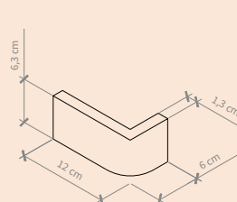
V. BRICK TRANSITION LEFT CORNER
