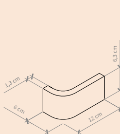
VICTORIAN BRICK CURVED CORNER
