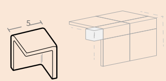
V-CAP CORNER OUTSIDE
